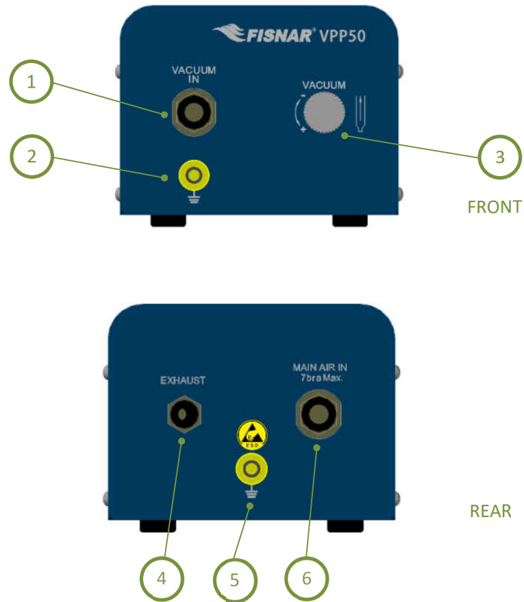
FIG. 1: External Controls – Overview
